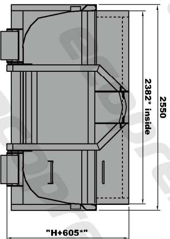
CLM12/6000D Combined top and side opening door with pneumatic/hydraulic flap locking
