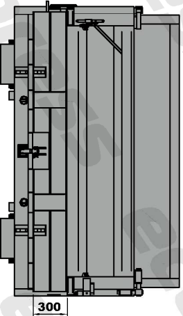
CLM12/6000D Combined top and side opening door with pneumatic/hydraulic flap locking
